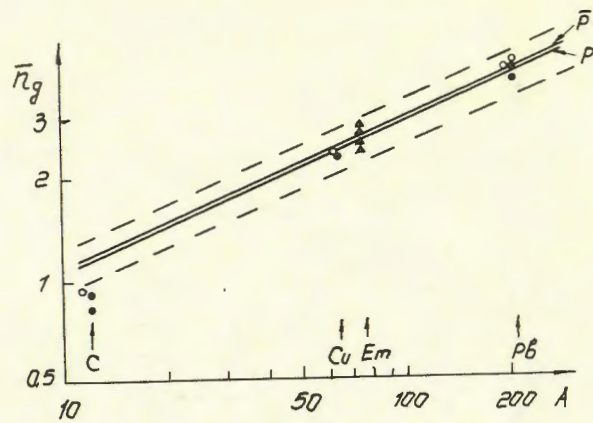
Fig. 3. Mean multiplicity of g-particles in p(\bar{p})A interactions: \bullet pA (50-150 GeV) [2]; \circ \bar{p}A (50-150 GeV) [2]; \blacktriangle pEm (50-400 GeV) [1]; lines present theoretical calculations according to the expression (9).
