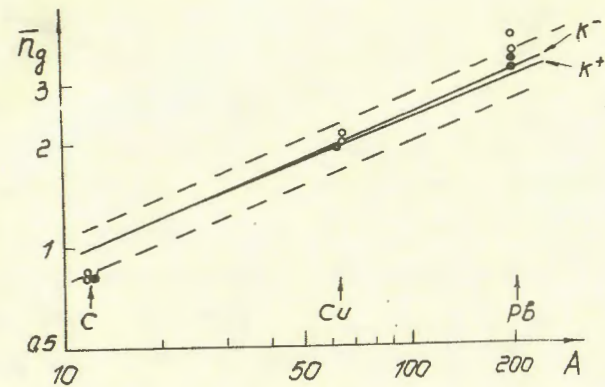
Fig. 2. Mean multiplicity of g-particles in K^+ A interactions: \bullet K^+ A (50 - 150 GeV) [2]; \circ K^- A (50 - 150 GeV) [2]; lines present theoretical calculations according to the expression (9).
