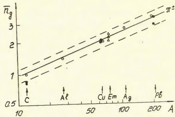
Fig. 1. Mean multiplicity of g-particles in \pi^+ A interactions: \bullet \pi^+ A (50-150 GeV) [2]; \circ \pi^+ A (37.5 GeV) [3]; \Delta \pi^- Em (50-340 GeV) [1]; lines present theoretical calculations according to the expression (8).
